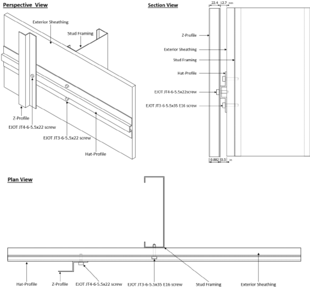
FIGURE 1 SWISSPEARL FIBER-CEMENT PANEL SYSTEM
